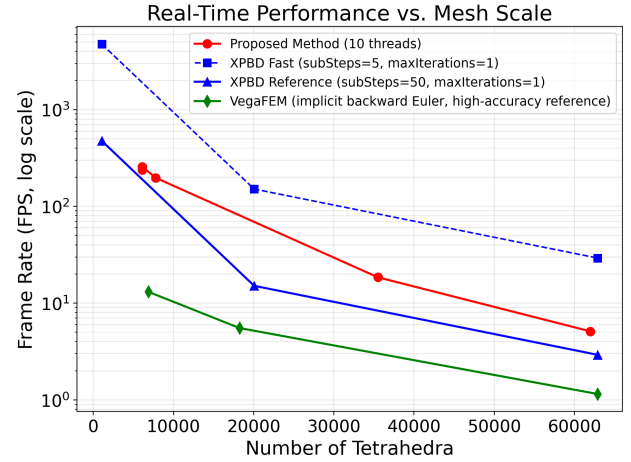
FIGURE 7. Overall performance trend across Frame rate versus mesh scale (log-scale FPS axis) for the proposed method (10 threads), XPBD under the Fast and Reference substep configurations defined in Section IV-A, and VegaFEM. The proposed method maintains better real-time performance than VegaFEM over a broad tetrahedral range and still retains basic interactivity on larger-scale models.
